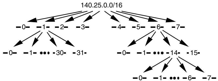
FIGURE D-1. Address Strategy for VLSM Example
